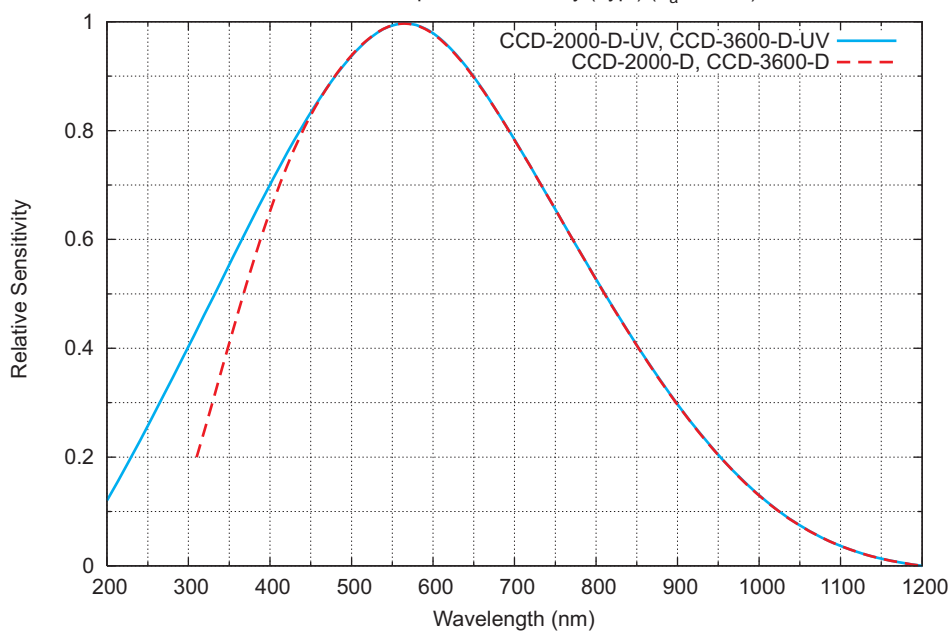
Normalized Spectral Sensitivity (Typ.) ( T_a = 25^\circ\text{C} )
